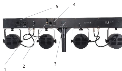
REAR VIEW 1 – Switch ON/OFF 2 – Antenna 3 – Display 4 – Power IN/OUT 5 – DMX in/OUT
