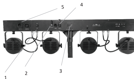
VISTA POSTERIORE 1 – Interruttore ON/OFF 2 – Antenna 3 – Display 4 – Power IN/OUT 5 – DMX in/OUT
