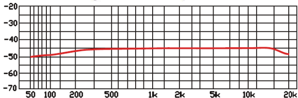
Figure 2: Frequencyresponse
