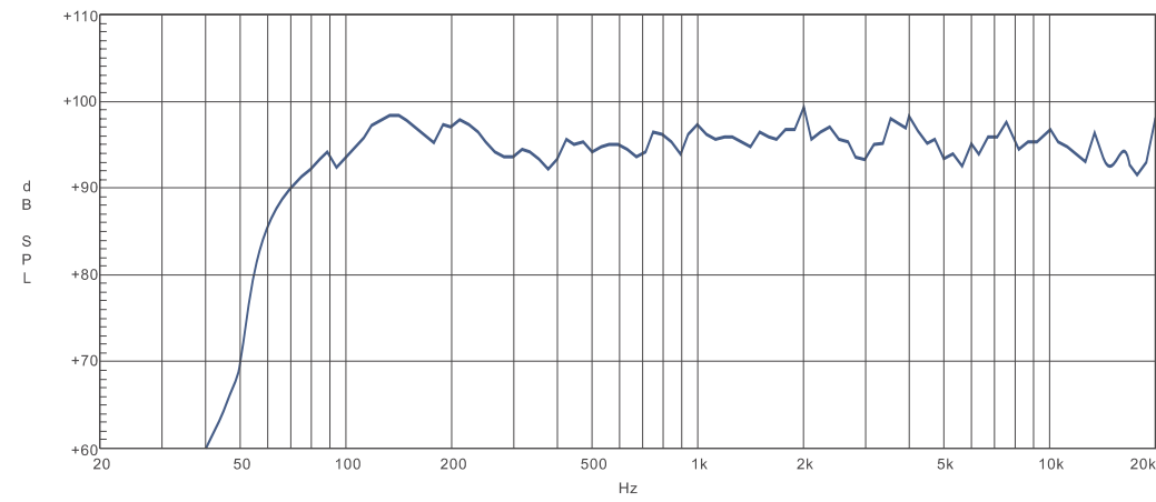
TPS i28H
