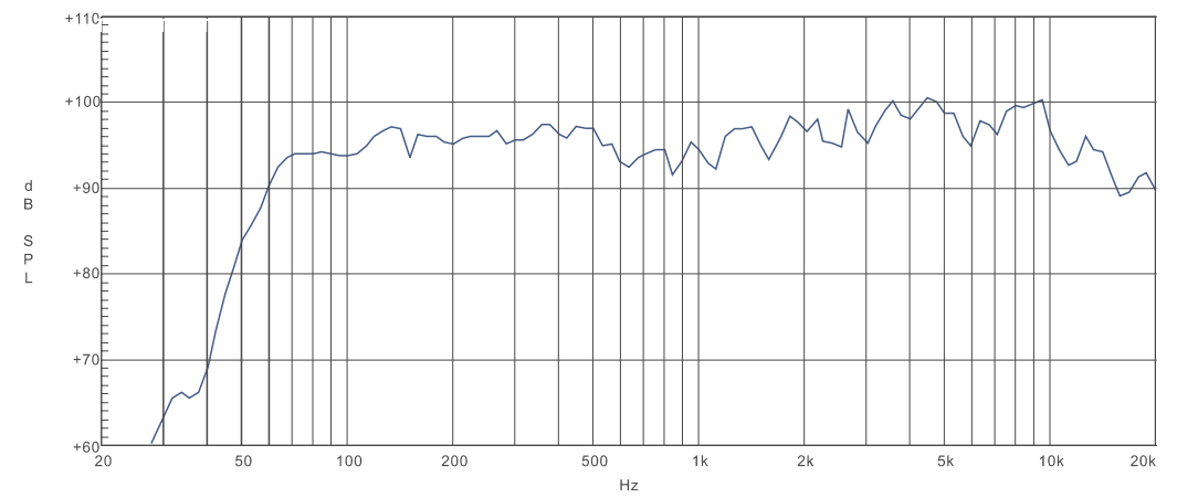
TPS i10HA
