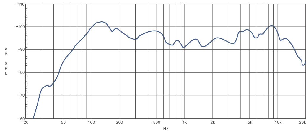
TPS i210H
