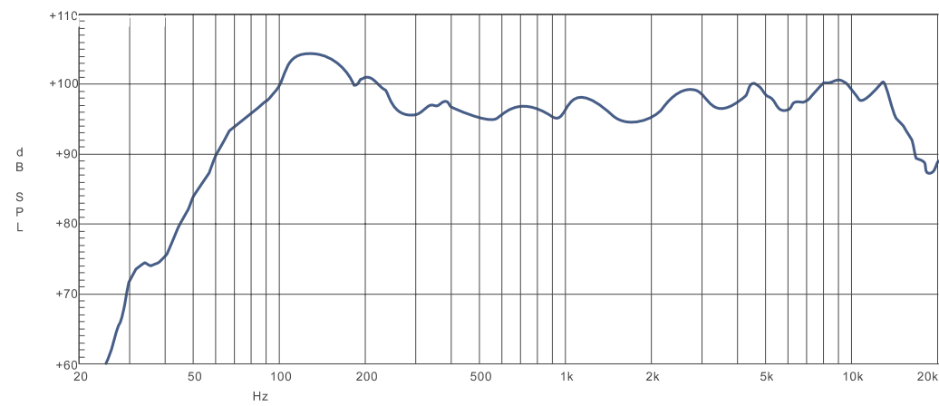
TPS i210HA
