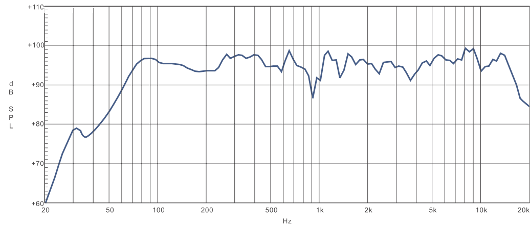
TPS i15HA
