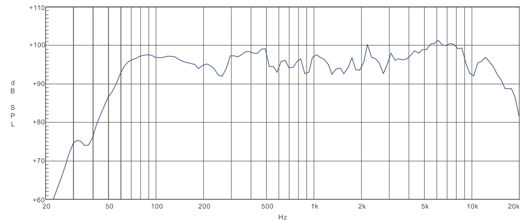
TPS i12HA
