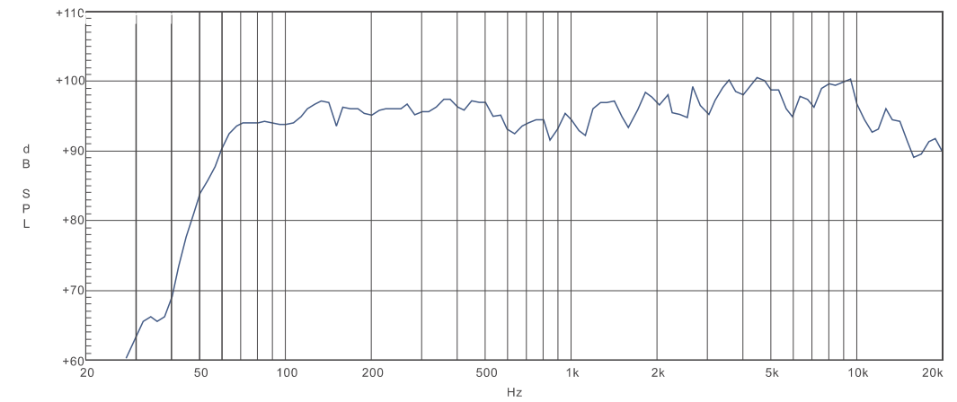
TPS i10H
