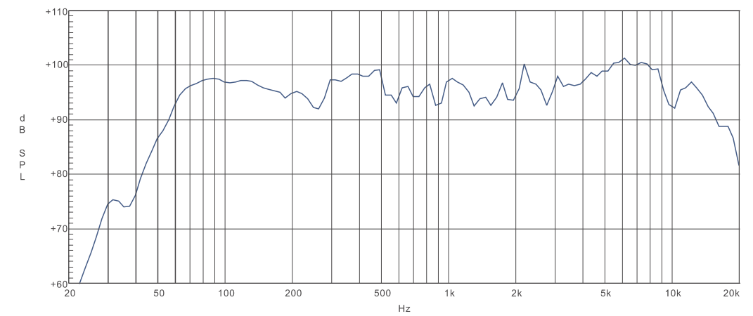
TPS i12HA
