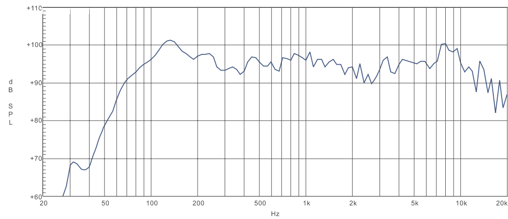
TPS i28HA
