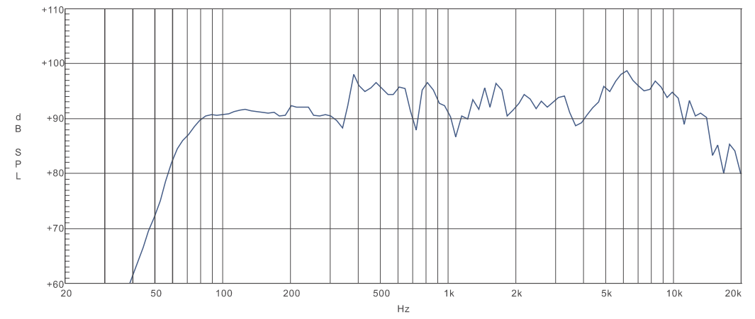
TPS i8HA
