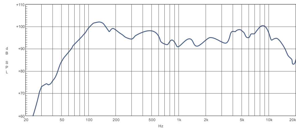
TPS i210H
