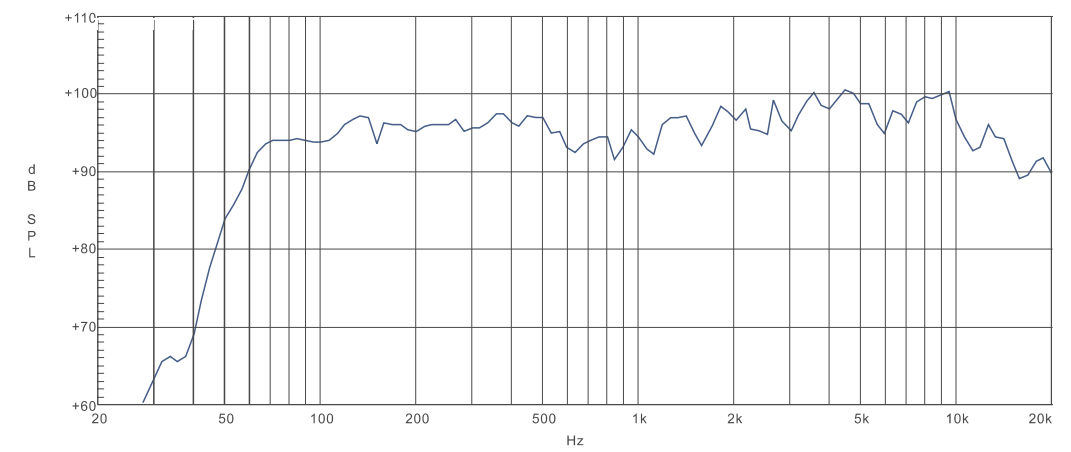
TPS i10HA
